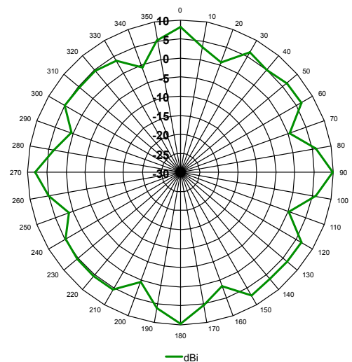
5.8GHz Azimuth Radiation Pattern
