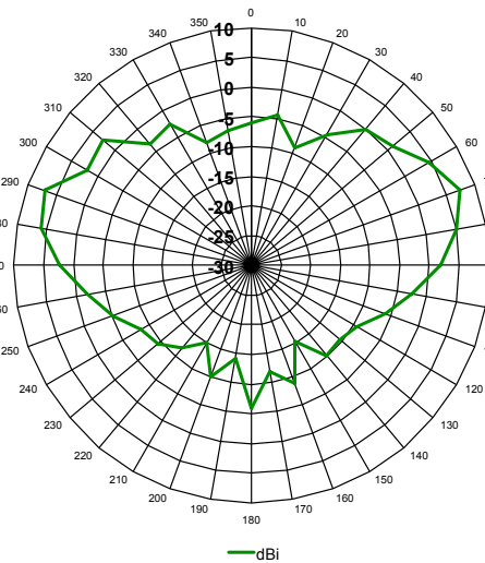
5.8GHz Elevation Radiation Pattern
