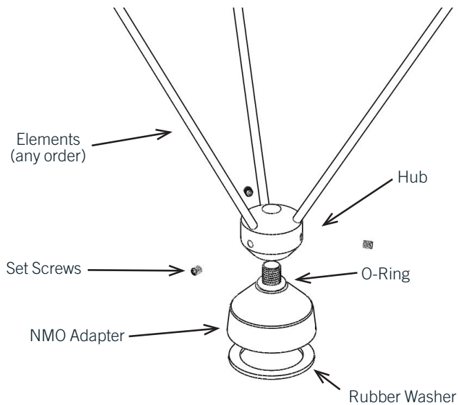
EXPANDED VIEW
